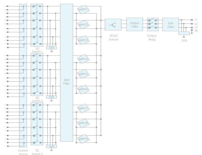
Circuit Diagram
