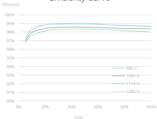
Efficiency Curve
